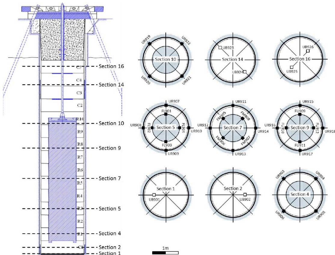
Figure 2.4 - Cross-section of the LASGIT deposition hole, showing the locations of monitoring cross-sections and the positions of technologies within these cross-sections (black and white squares with labels beginning with U). In cross-sections 5, 7 and 9, pressure transducers associated with the hydration mats are positioned on the canister surface (black squares with labels beginning with F) [25].
