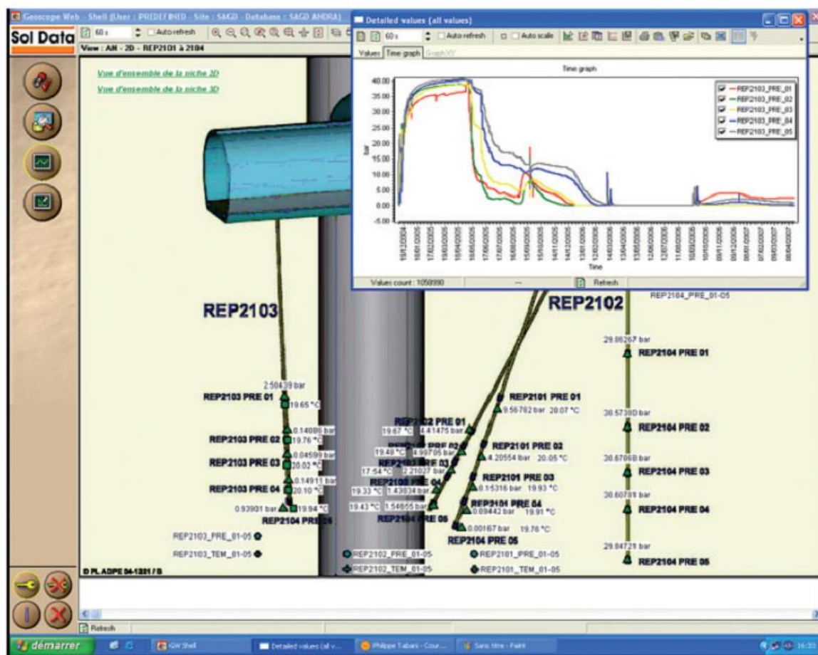
Figure 2.17 - Graph of pore pressure data over time at multiple locations, along with a visualisation of the sensor location, taken from the Geoscope web interface, used by Andra in the ALC1605 demonstrator [3].
